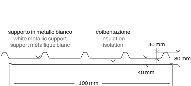
Pannello coibentato Insulated panel Panneau isolant
